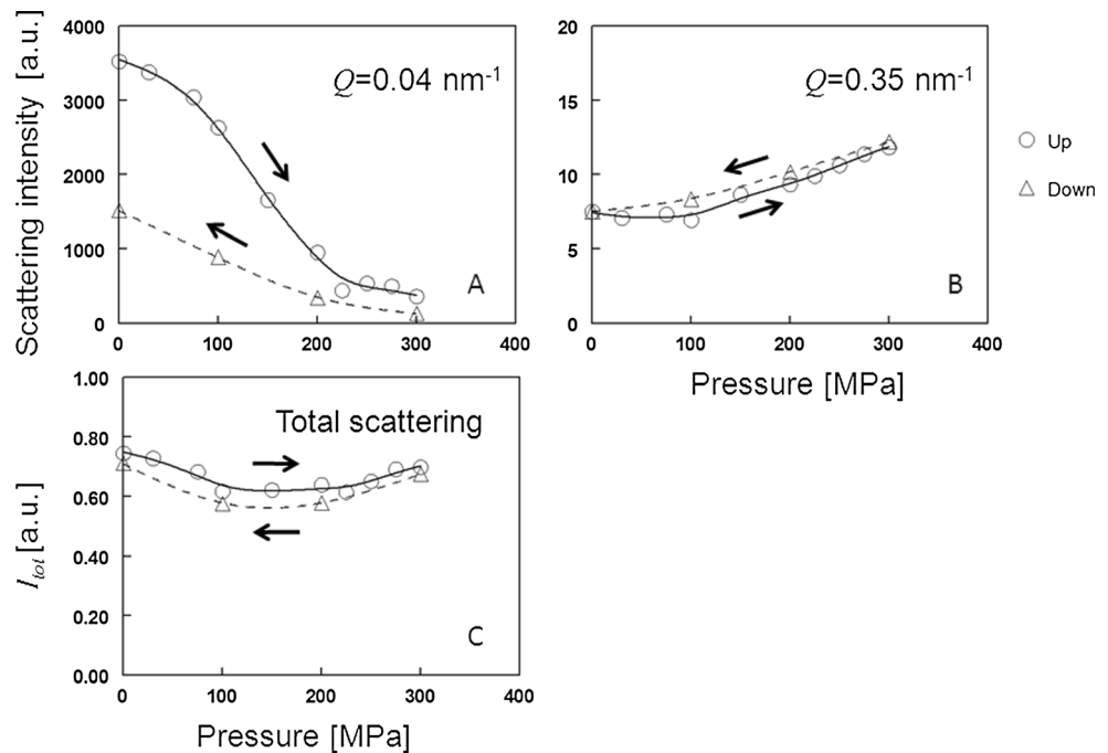
Fig. 2 The scattering intensity at low (a) and high (b) Q values with increasing and decreasing pressure, and total scattering (c). The curves are aides to the eye. Downward: equilibration at 300 MPa and stepwise descend to ambient pressure; Upward: stepwise ascend from ambient pressure to 300 MPa. Time step approx. 1 h. It should be noted that the upward and downward pressure series were recorded with different samples.
